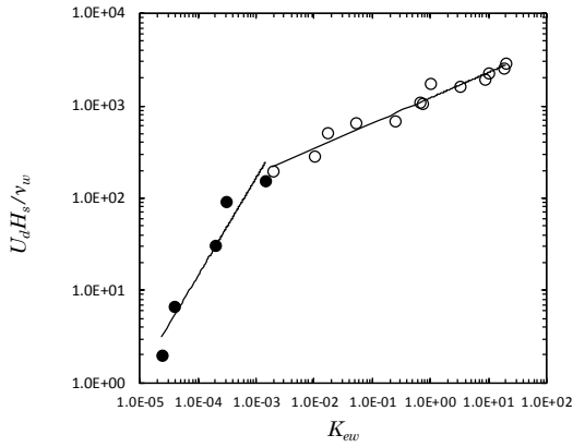
Fig. 5 Relation between U_d H_s / v_w and K_{ew}
