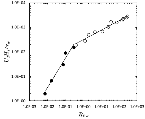
Fig. 6 Relation between U_d H_s / v_w and R_{Bw}
