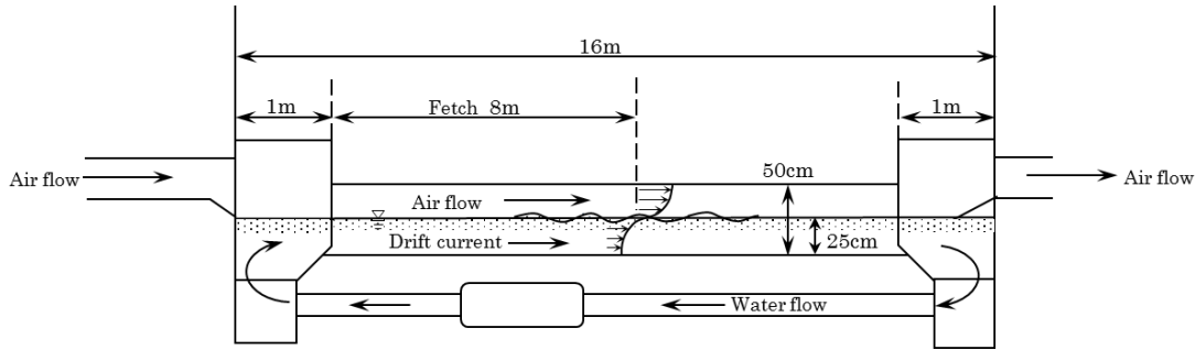
Fig. 1 Experimental apparatus
