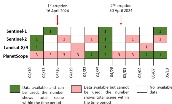
Fig. 3: Remote sensing data availability for 2024 Ruang Volcano eruption from 10 April to 10 May 2024
