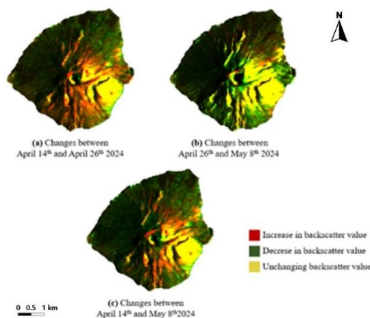
Fig. 7: Backscatter value changes between pre-eruption date and post-eruption dates
