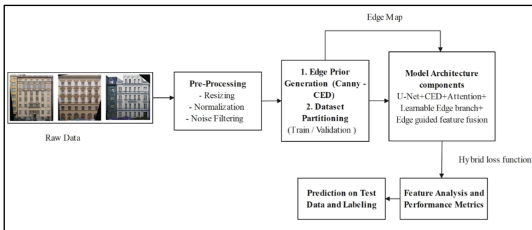
Fig. 3: Pipeline of Layered Framework
