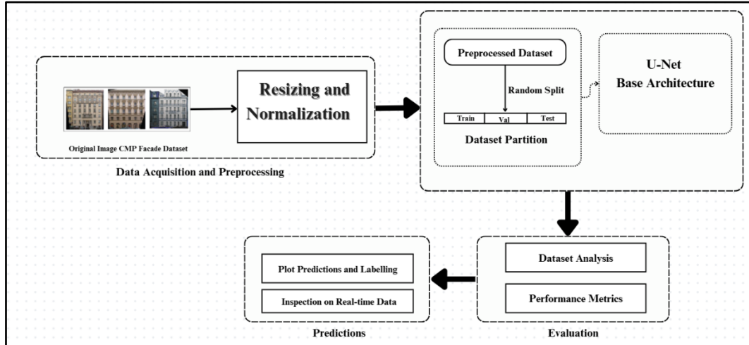
Fig. 2: Pipeline of Basic Network
