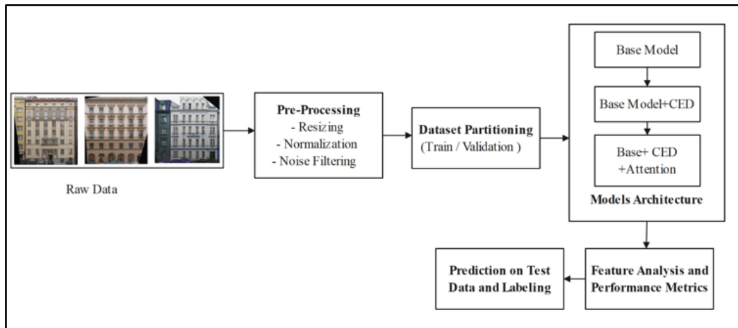
Fig. 3: Pipeline of Layered Framework
