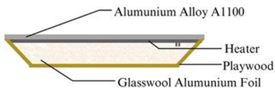
Fig. 3: Solar PV Model
