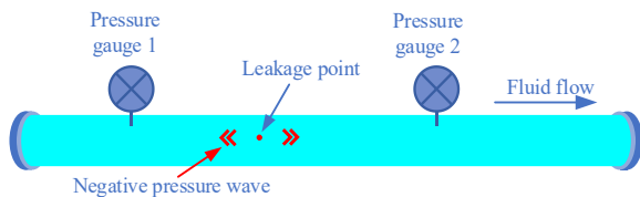
Fig. 5: Schematic principle of pressure monitoring for leakage detection
