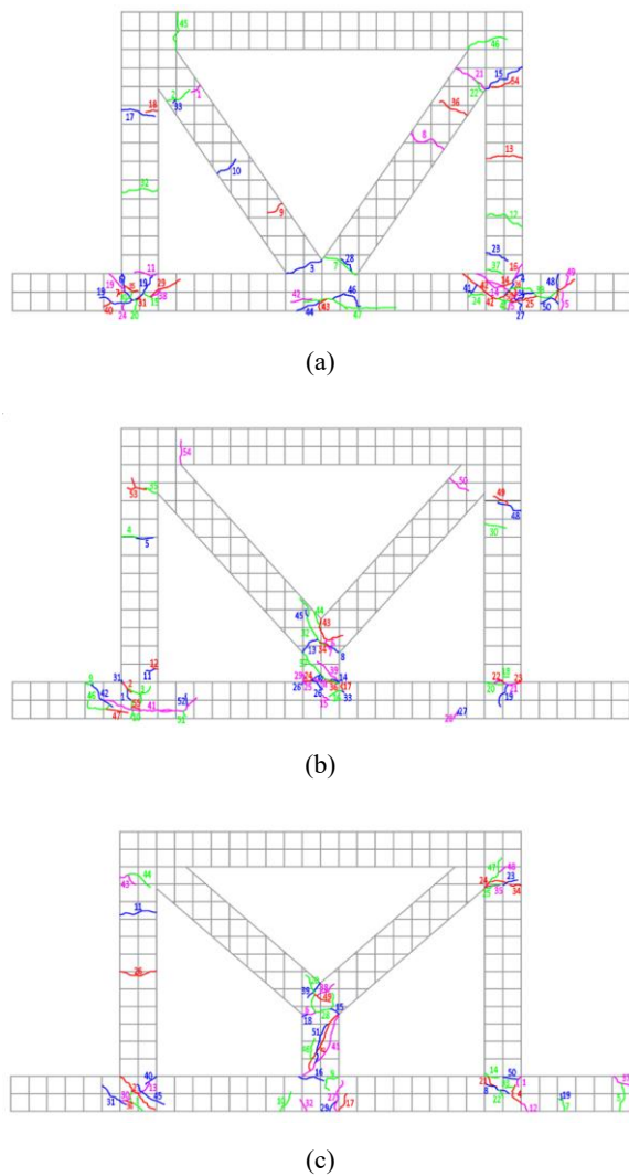
Fig. 10: Crack pattern of frame: (a) CBF, (b) EBF-V-15, (c) EBF-V-25
