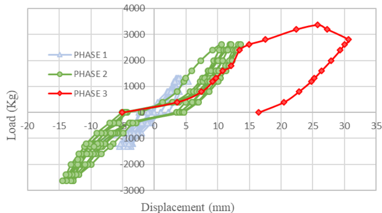
Fig. 4: Hysteresis curve of V-type concentrically reinforced frame
