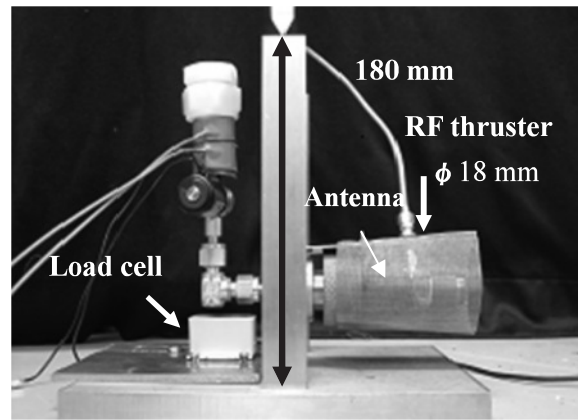
Fig. 3 Thrust stand for thrust measurement.
