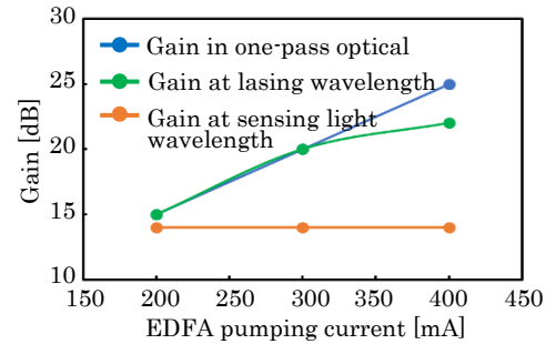
Fig. 4 EDFA gain at self-lasing wavelength, signal wavelength, and in single pass optical system.
